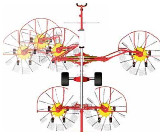
Infinitely variable hydraulic working width adjustment
